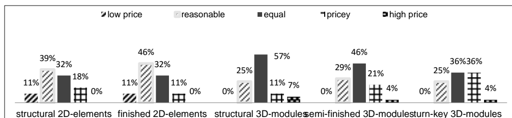
Figure 3. Expert survey cost comparison of traditional to industrialized building systems (Hintersteiner 2015).
