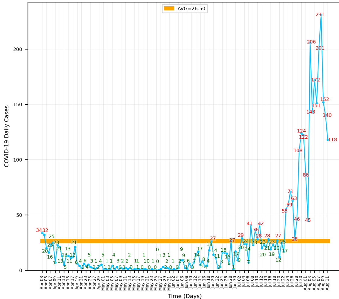
'Modified' Control Chart of COVID-19 Daily Cases in HAWAII (Apr 03, 2020 - Aug 11, 2020)
