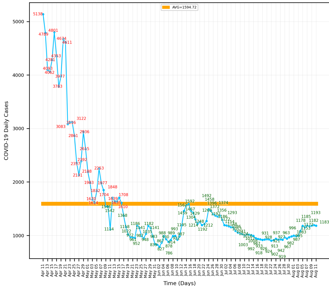
'Modified' Control Chart of COVID-19 Daily Cases in TURKEY (Apr 11, 2020 - Aug 11, 2020)
