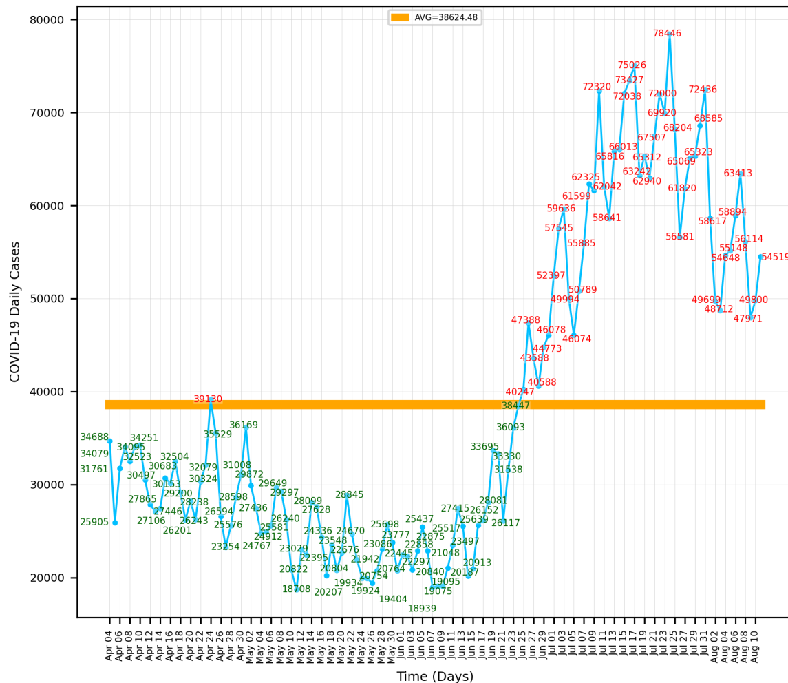
'Modified' Control Chart of COVID-19 Daily Cases in USA (Apr 04, 2020 - Aug 11, 2020)
