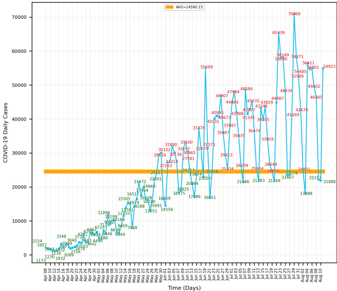
'Modified' Control Chart of COVID-19 Daily Cases in BRAZIL (Apr 08, 2020 - Aug 11, 2020)
