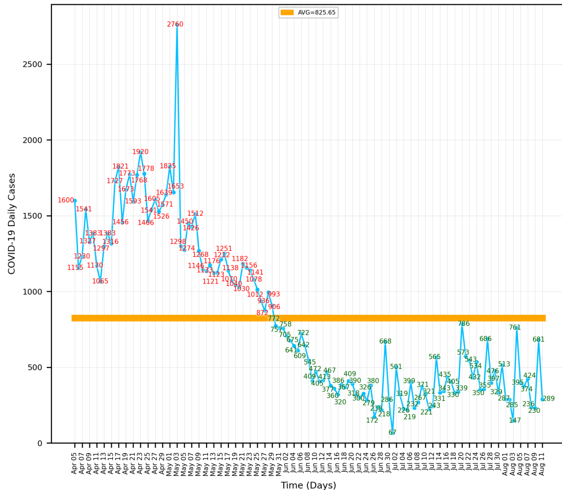
'Modified' Control Chart of COVID-19 Daily Cases in CANADA (Apr 05, 2020 - Aug 11, 2020)
