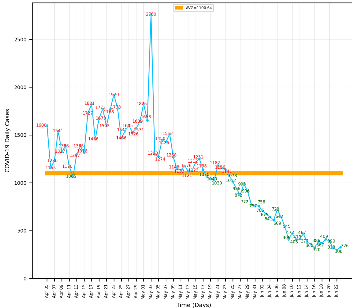
'Modified' Control Chart of COVID-19 Daily Cases in CANADA (Apr 05, 2020 - Jun 23, 2020)
