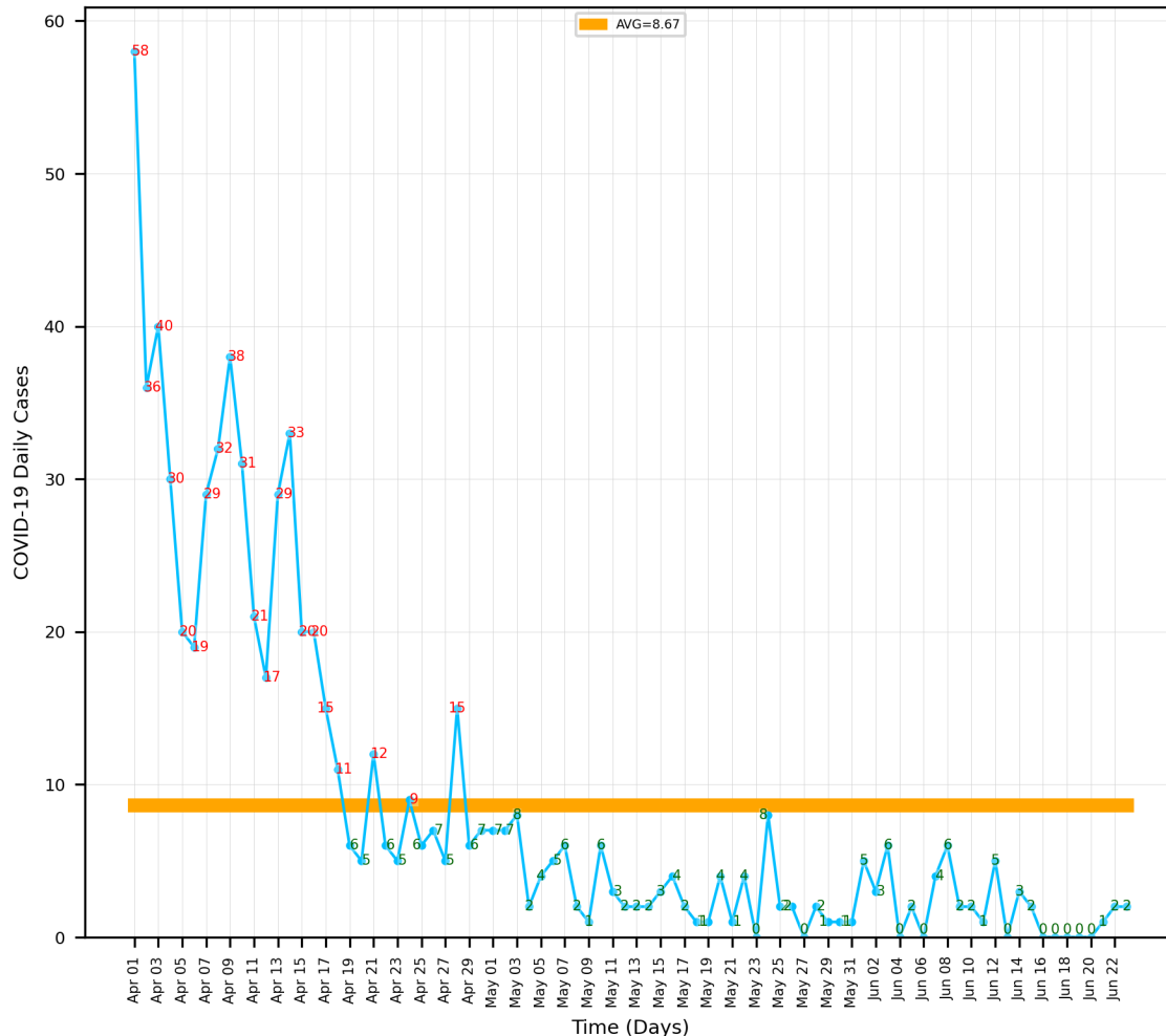
'Modified' Control Chart of COVID-19 Daily Cases in CYPRUS (Apr 01, 2020 - Jun 23, 2020)
