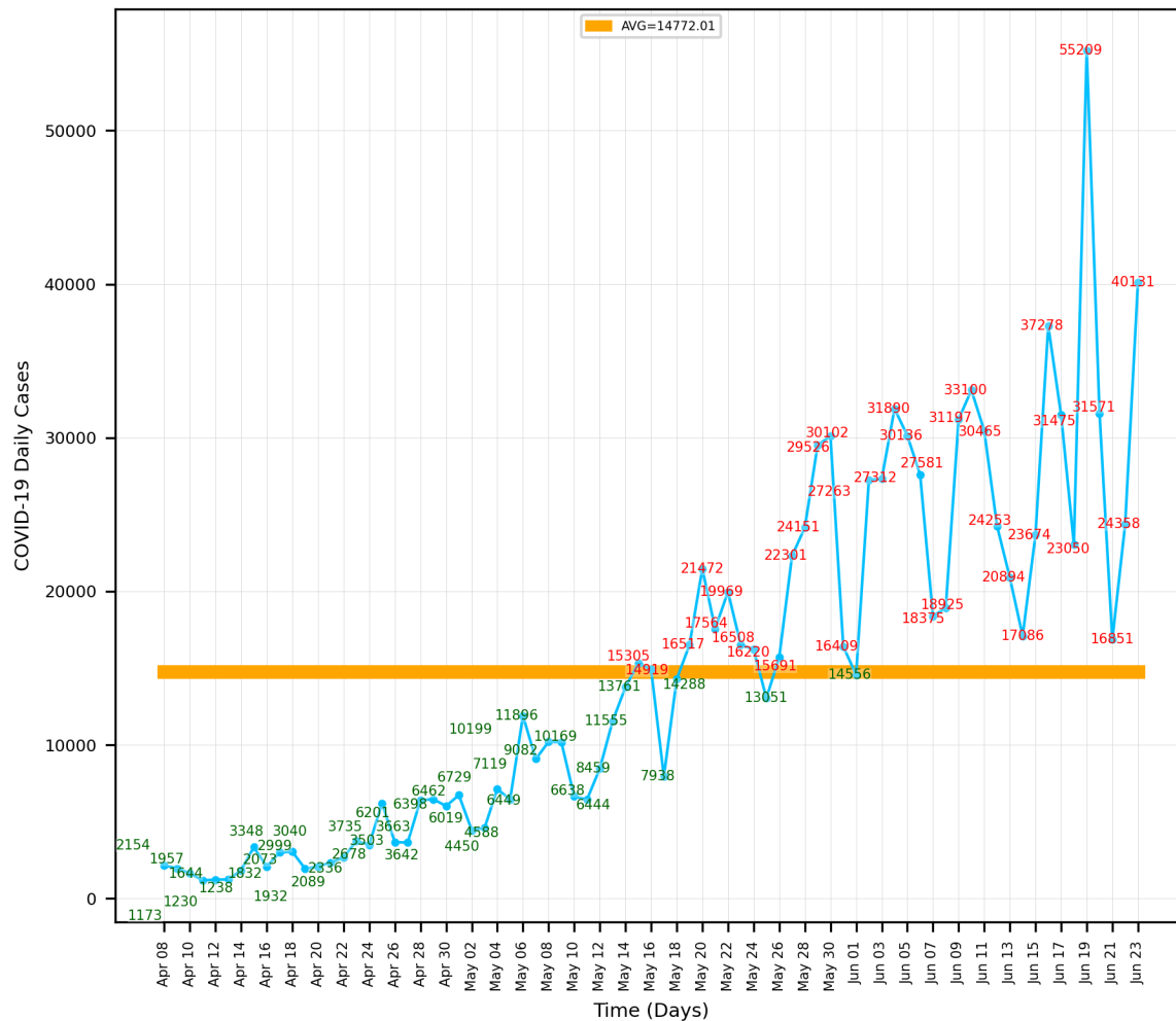
'Modified' Control Chart of COVID-19 Daily Cases in BRAZIL (Apr 08, 2020 - Jun 23, 2020)
