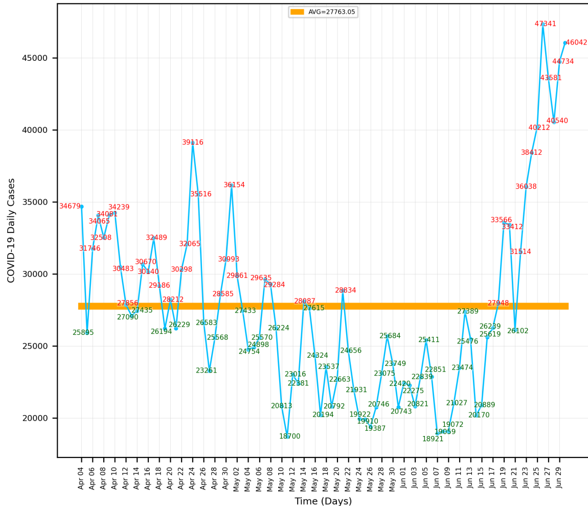
'Modified' Control Chart of COVID-19 Daily Cases in USA (Apr 04, 2020 - Jun 30, 2020)
