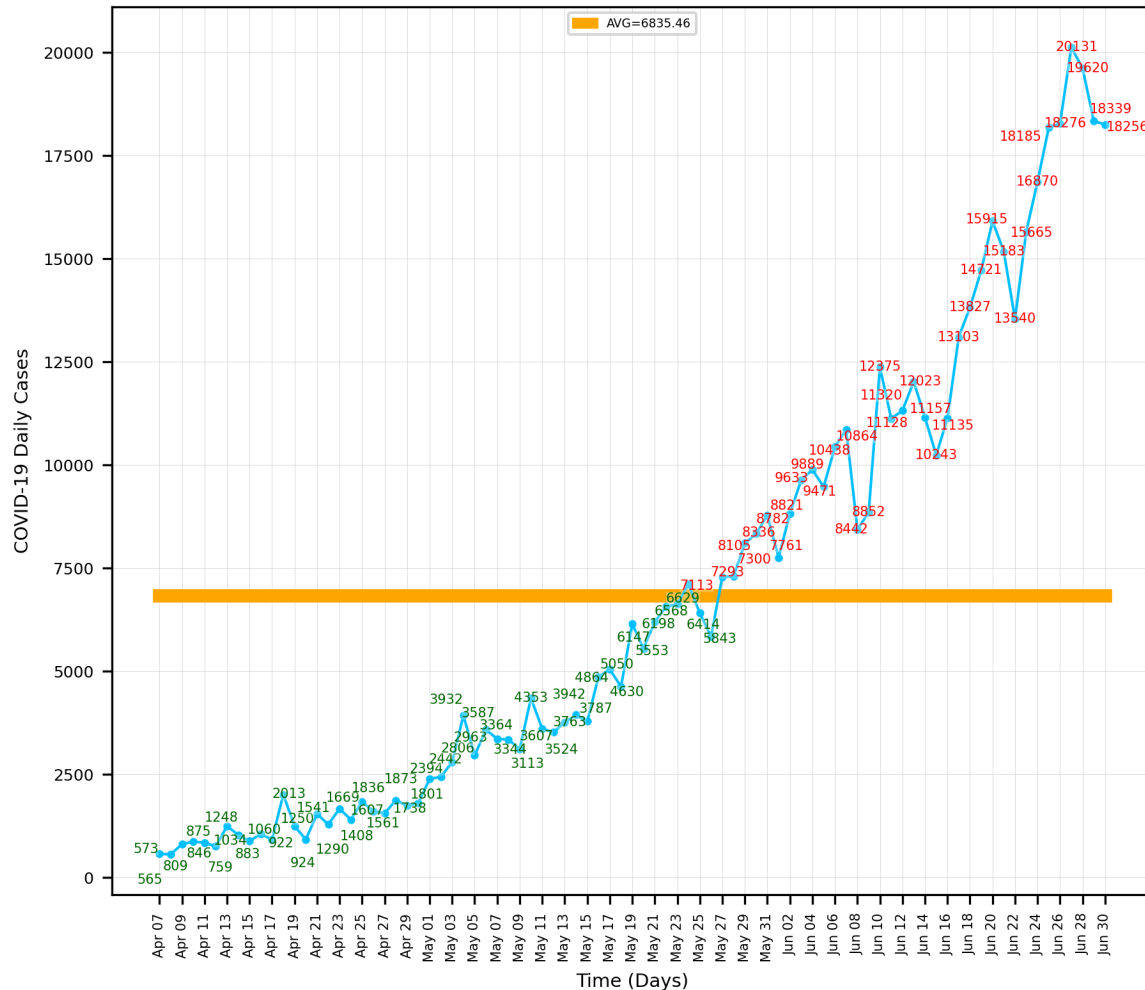
'Modified' Control Chart of COVID-19 Daily Cases in INDIA (Apr 07, 2020 - Jun 30, 2020)
