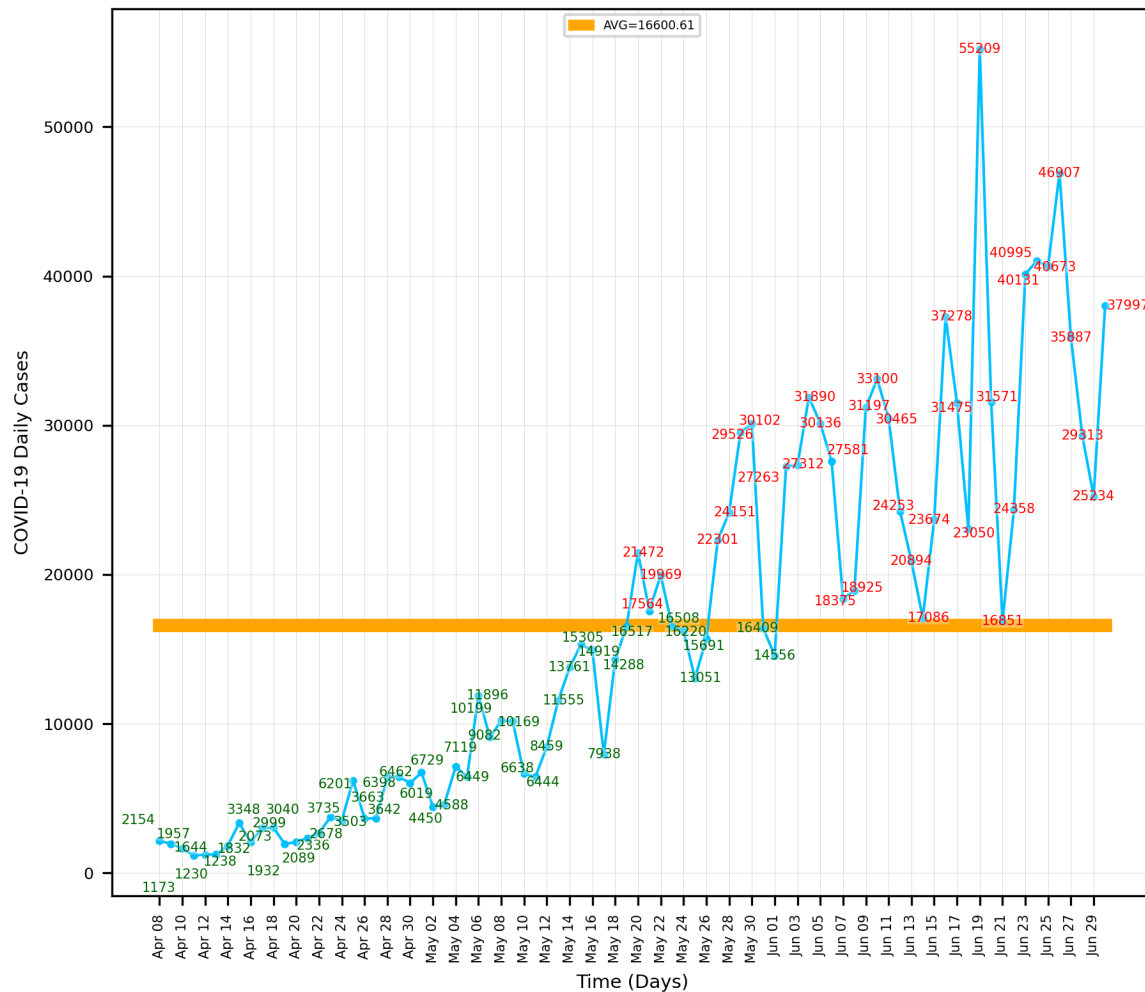
'Modified' Control Chart of COVID-19 Daily Cases in BRAZIL (Apr 08, 2020 - Jun 30, 2020)
