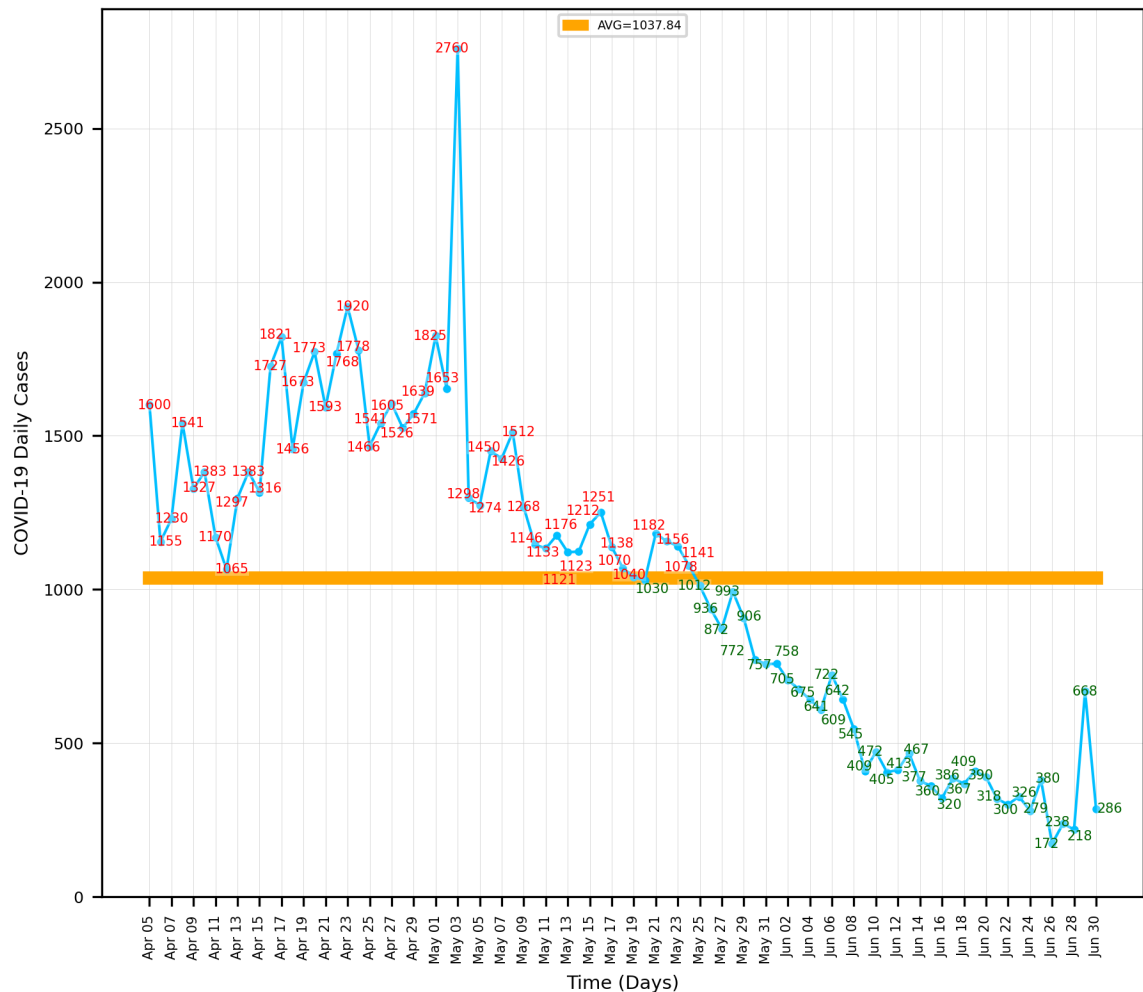
'Modified' Control Chart of COVID-19 Daily Cases in CANADA (Apr 05, 2020 - Jun 30, 2020)
