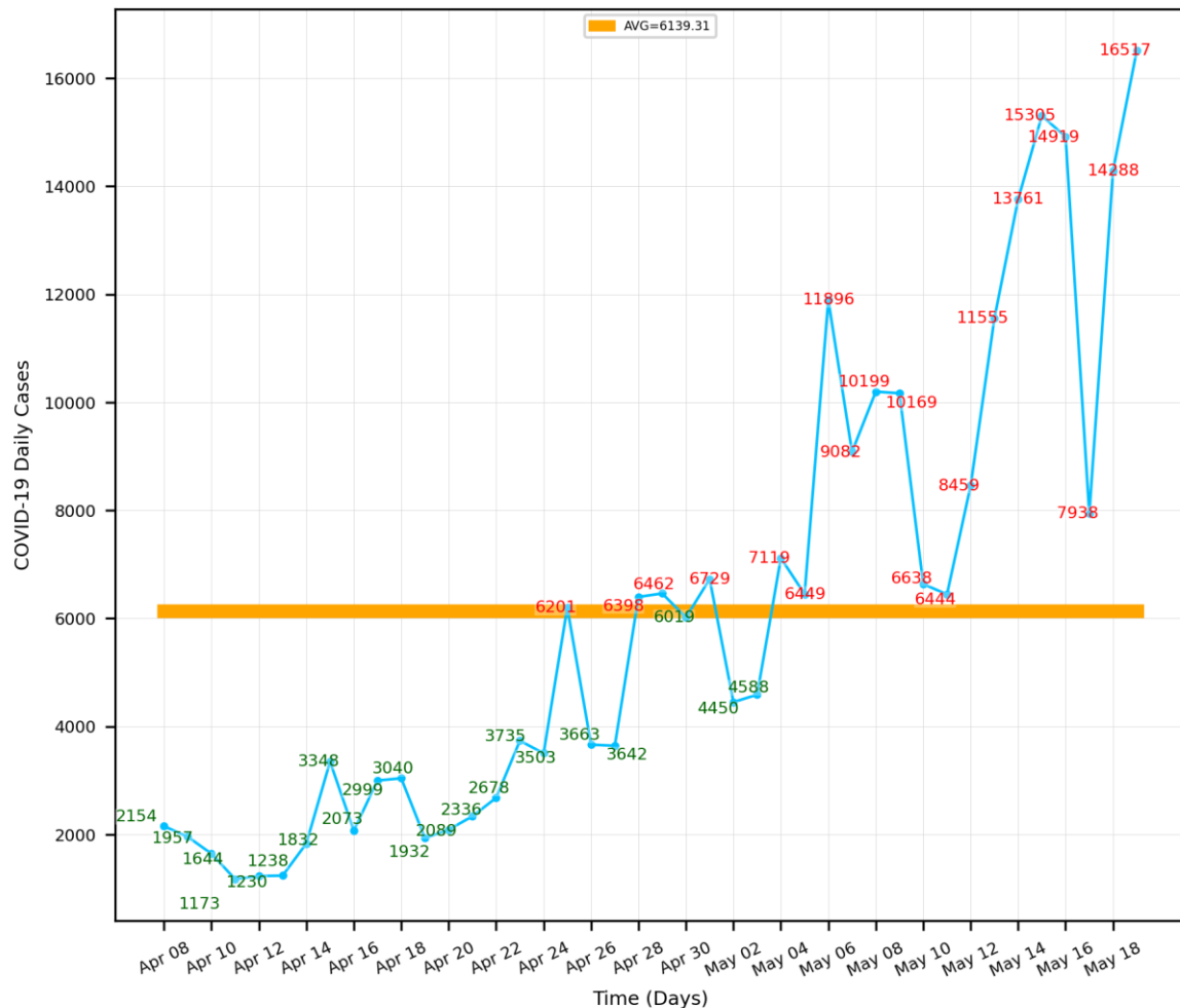
'Modified' Control Chart of COVID-19 Daily Cases in BRAZIL (Apr 08, 2020 - May 19, 2020)
