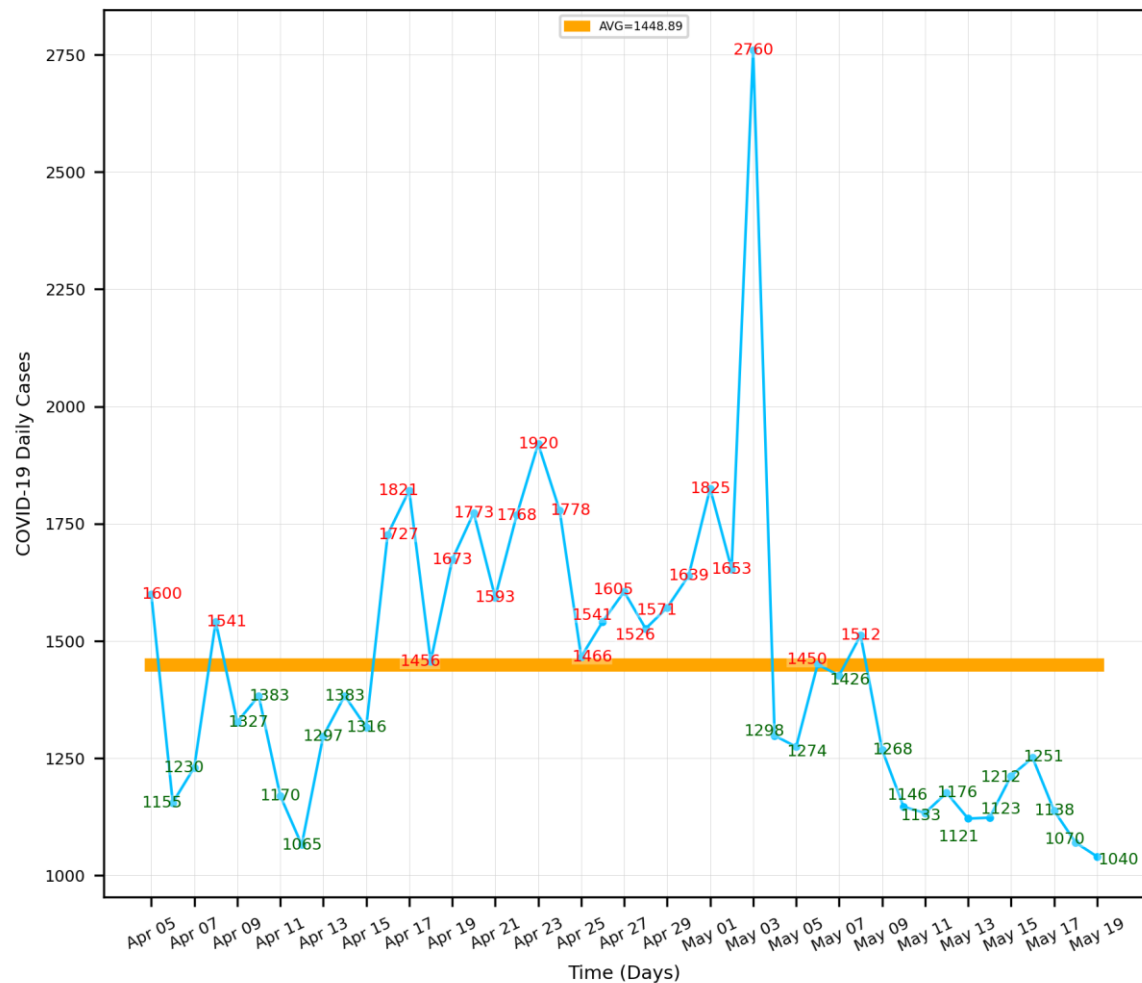
'Modified' Control Chart of COVID-19 Daily Cases in CANADA (Apr 05, 2020 - May 19, 2020)
