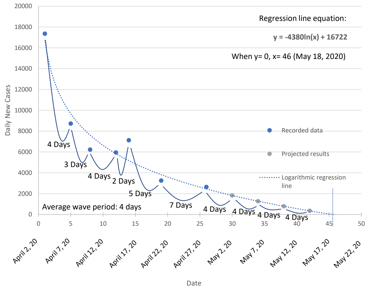
Regression Line for Peak Periods: France
